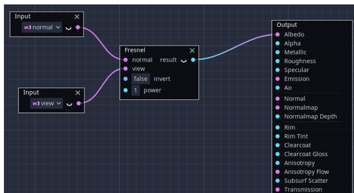
Figure 304: Godot’s “Visual Shader” Editor
